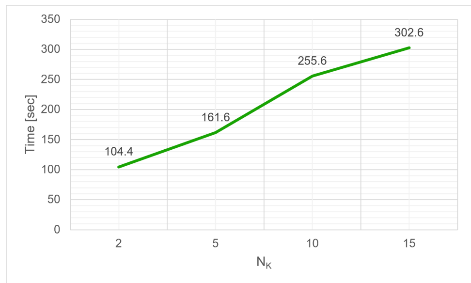
Figure 7. Execution time of the Standard technique for different values of N_K (Dermatology dataset).
