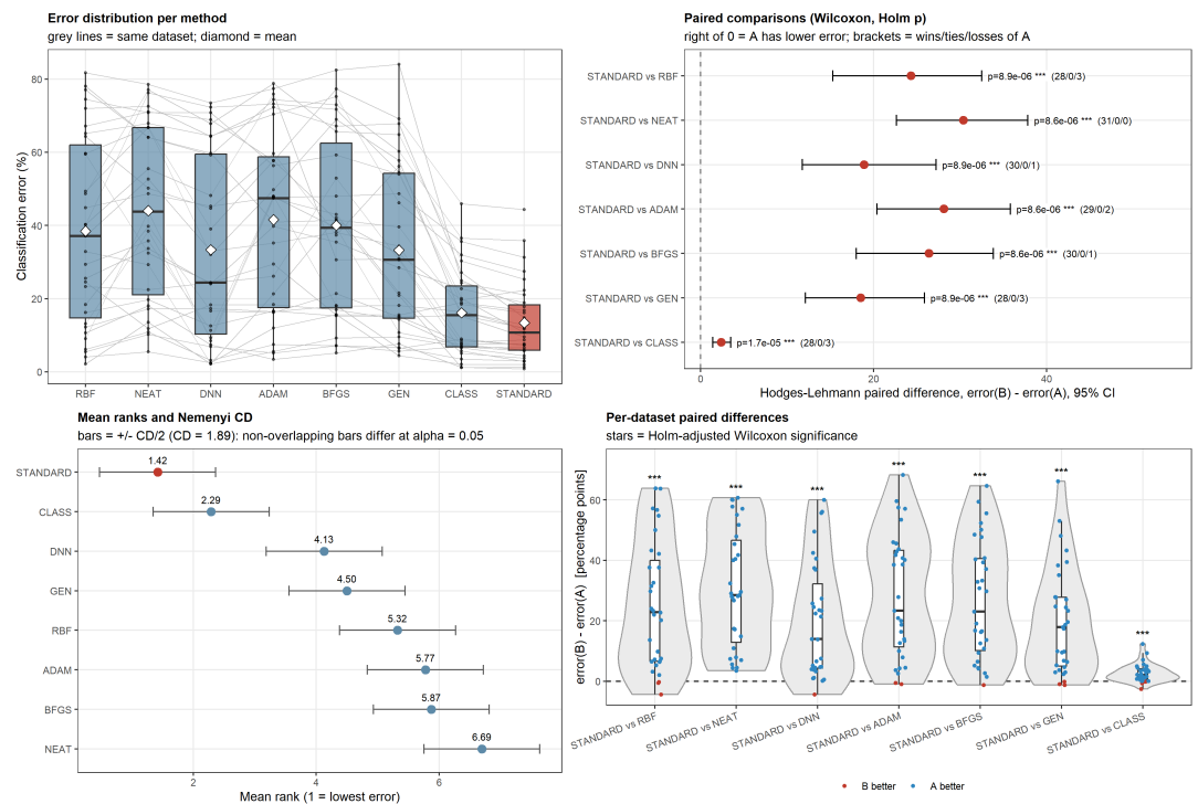
Figure 4. Statistical comparison of the proposed method (STANDARD) against the other classifiers over 31 datasets.
