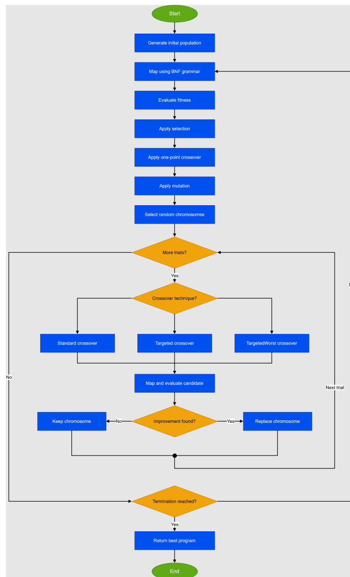
Figure 3. Flowchart of the proposed GenClass method with the additional crossover techniques.
