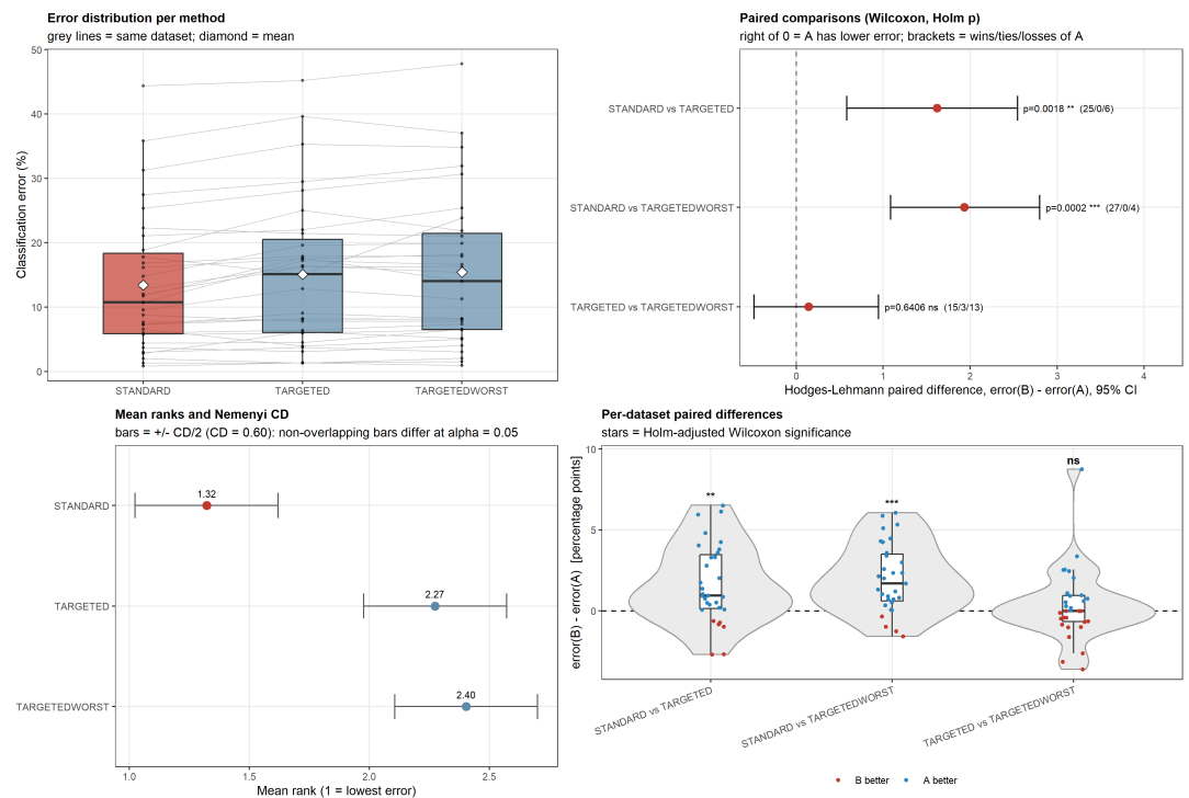
Figure 5. Statistical comparison of the three three crossover strategies. (STANDARD, TARGETED, TARGETEDWORST).
