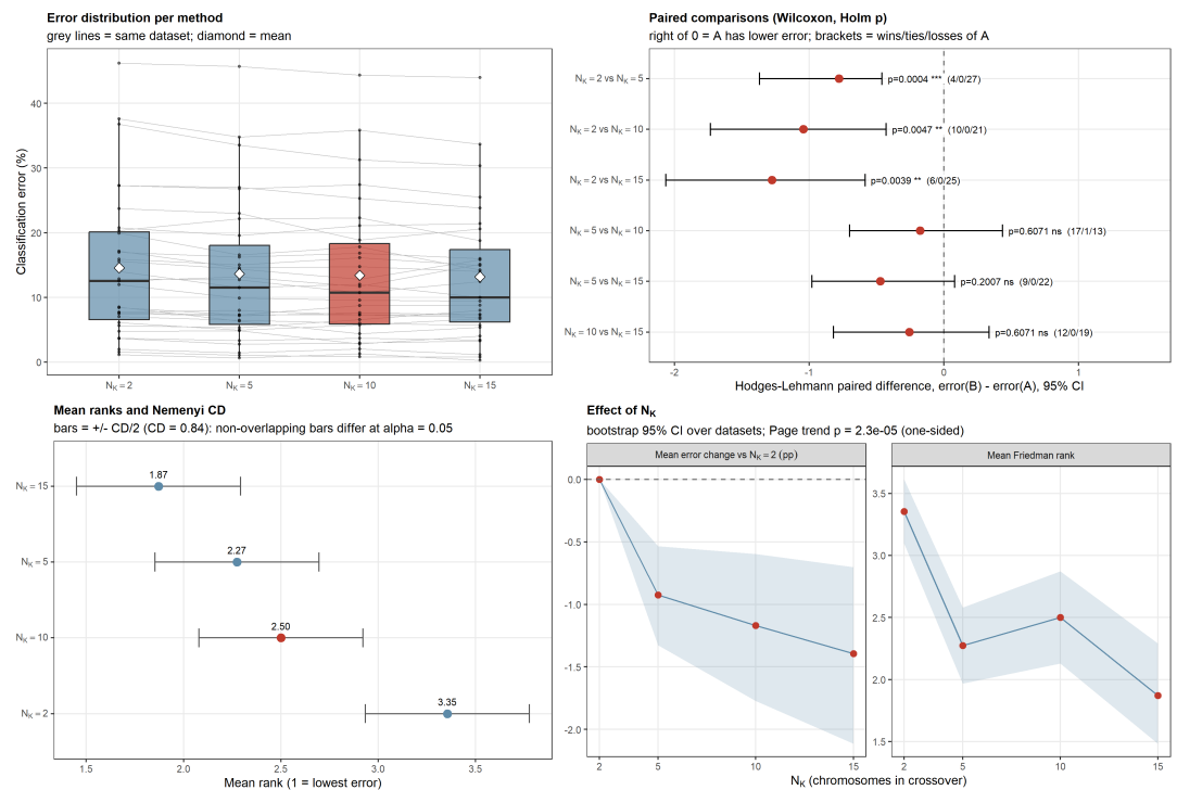
Figure 6. Effect of the number of chromosomes ( N_K ) participating in the crossover on the proposed method.
