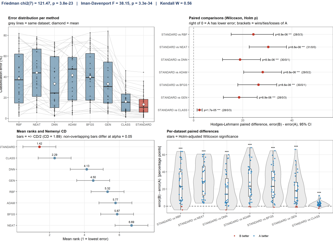
Figure 3. Statistical comparison of the proposed method (STANDARD) against the other classifiers over 31 datasets.
