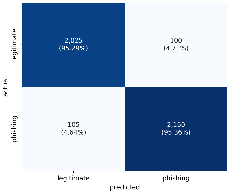
Confusion matrix, summed over five seeds: UCI Phishing Websites (de-duplicated) - Soft-voting ensemble.
