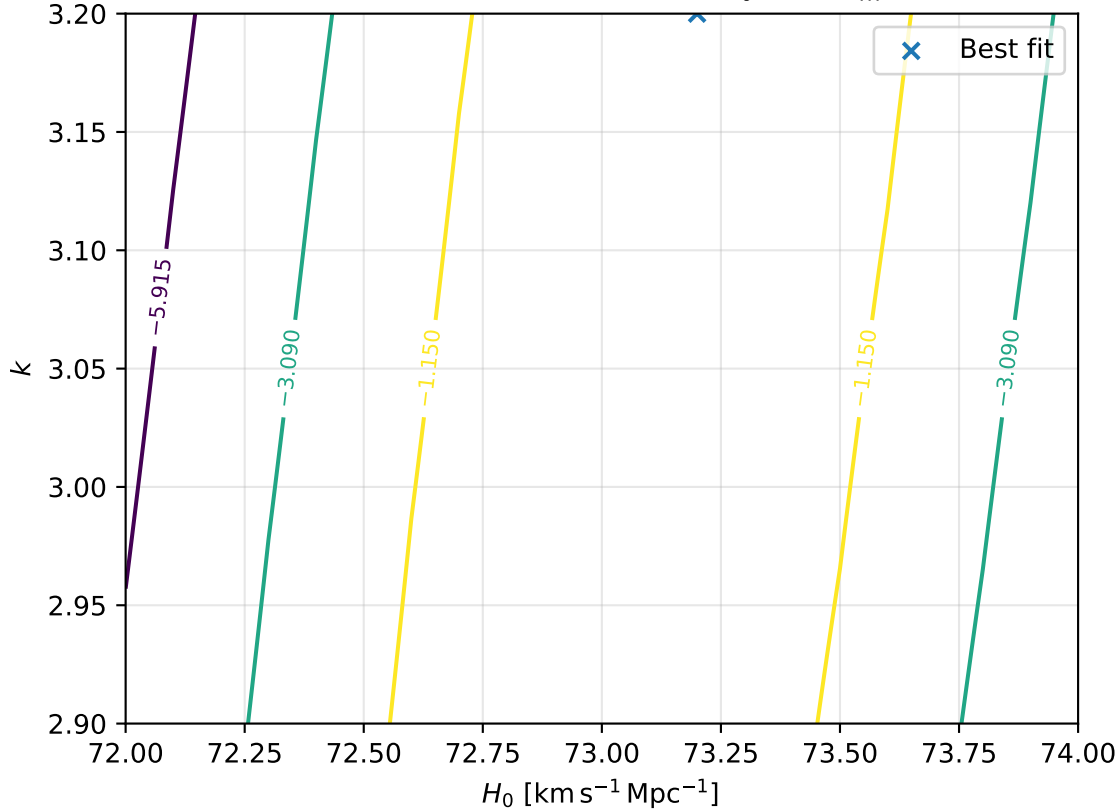
Pantheon+ Likelihood (CCBH) in (H_0, k) ( \Omega_m = 0.386 )
