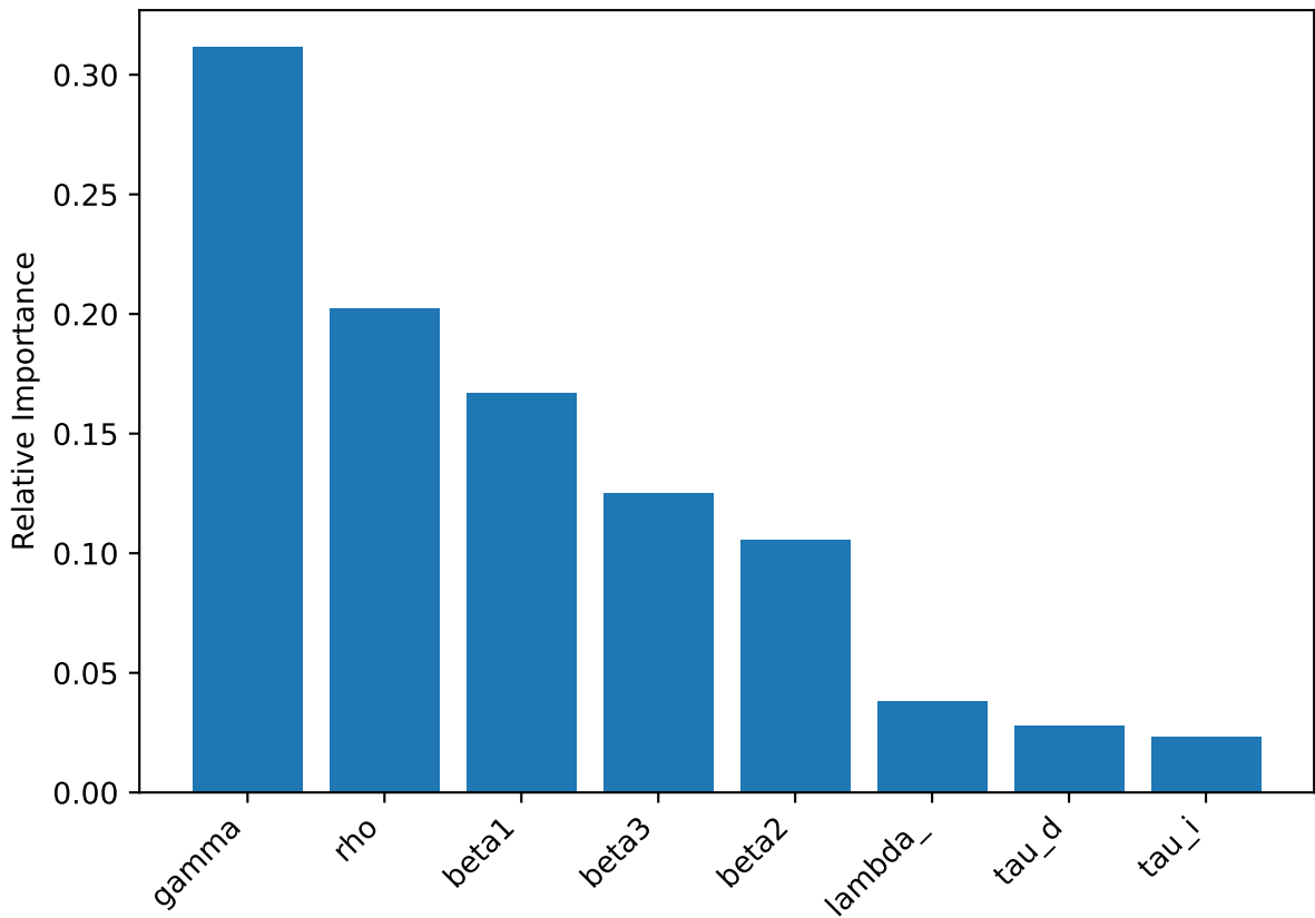
SMM Hyperparameter Importance
