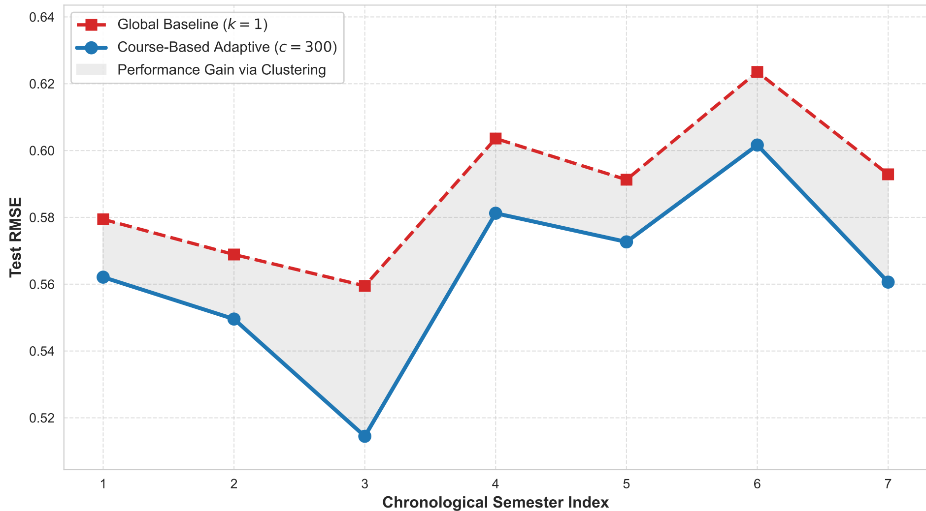
Temporal Error Trajectories: Global vs. Clustered Framework
