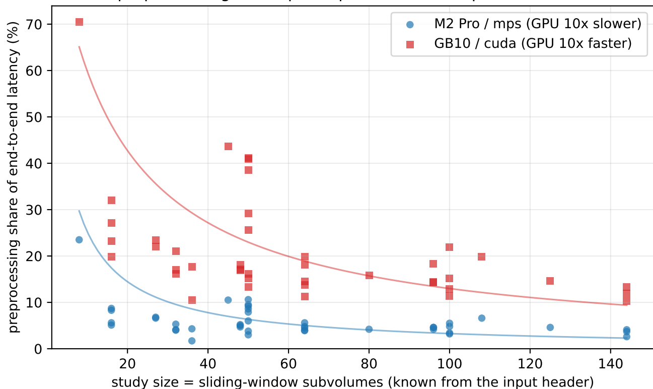
Excluded preprocessing is sample-dependent and amplifies on the faster GPU
