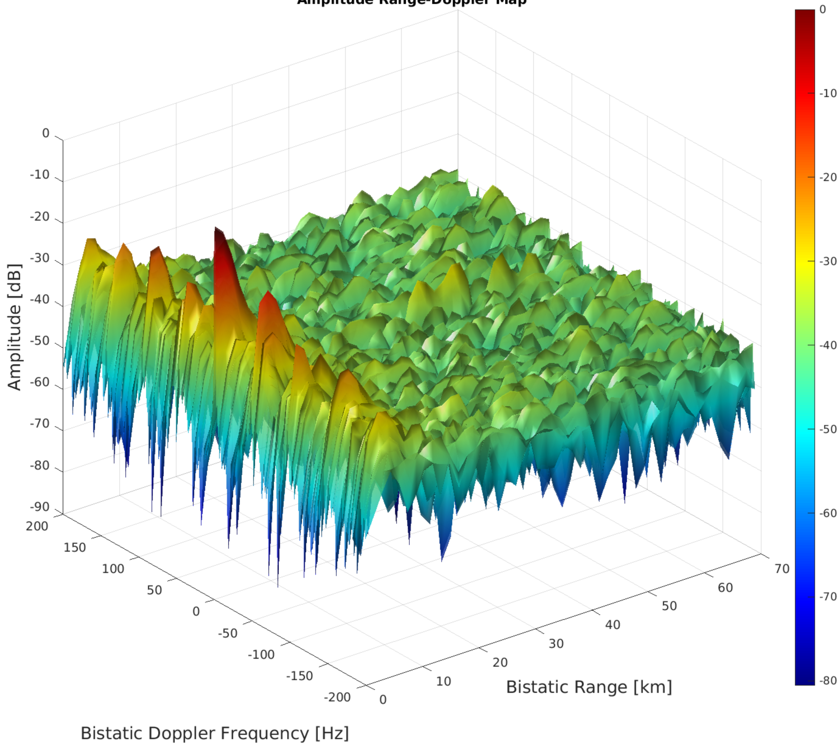
Amplitude Range-Doppler Map
