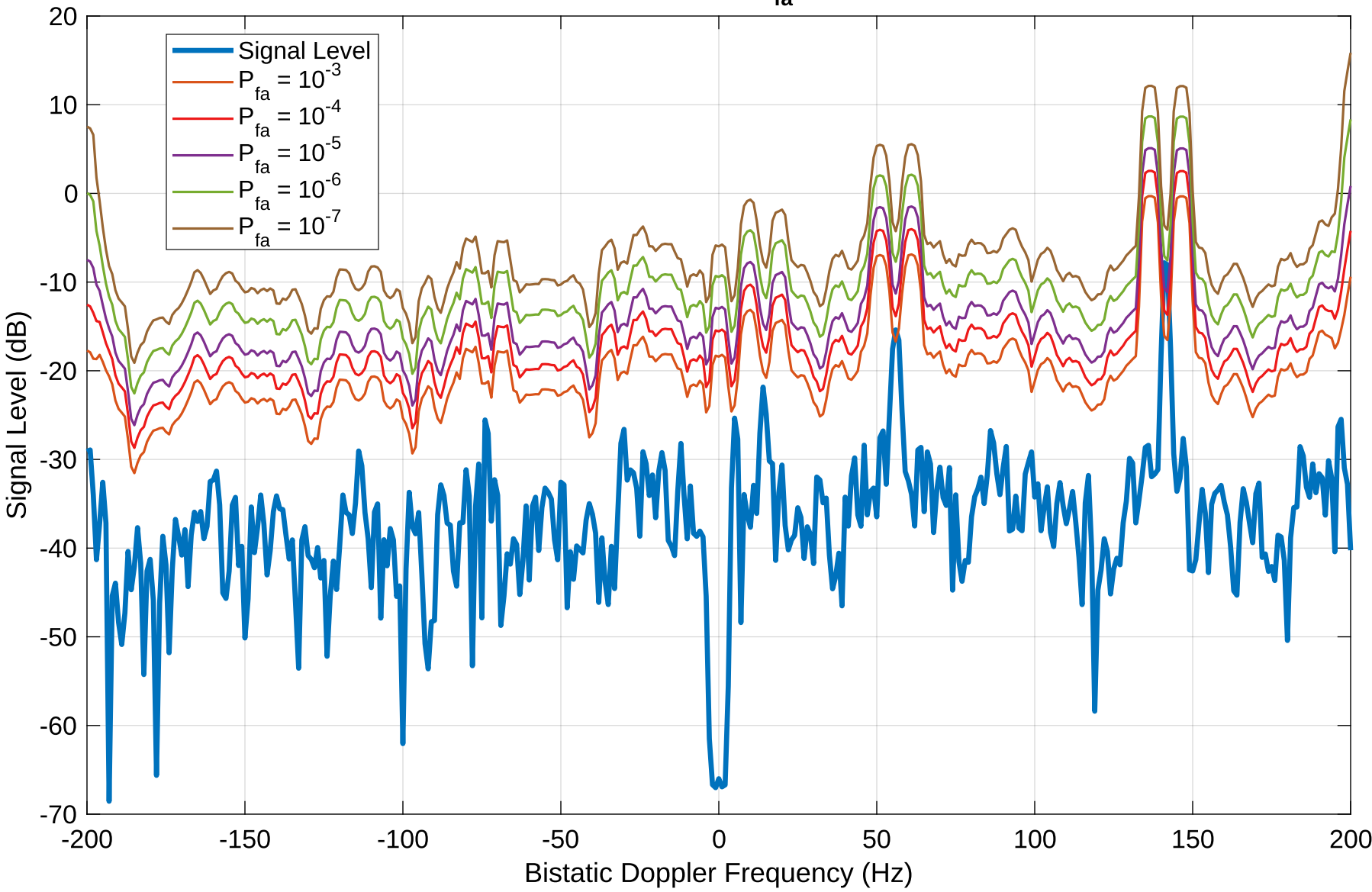
CA-CFAR Threshold with Different P_{fa} s — Bistatic Range: 15 km
