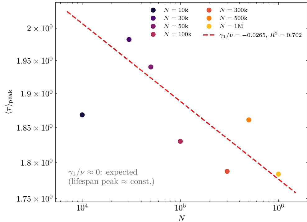
\gamma = 3.5 peak height
