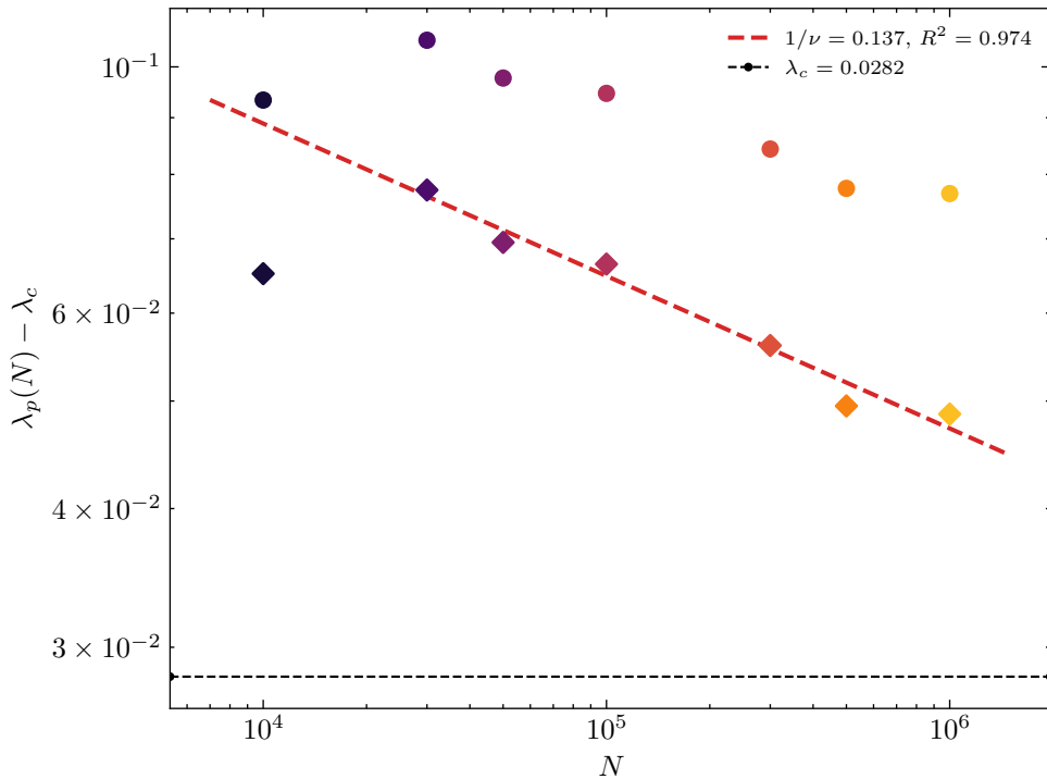
\gamma = 3.5 peak position
