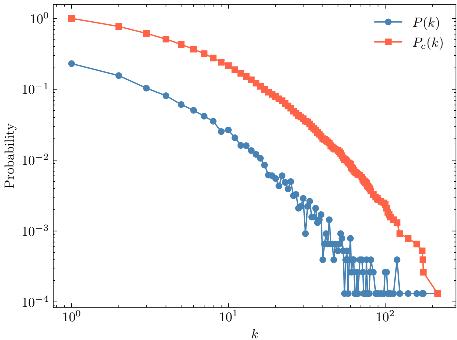
Degree distribution
