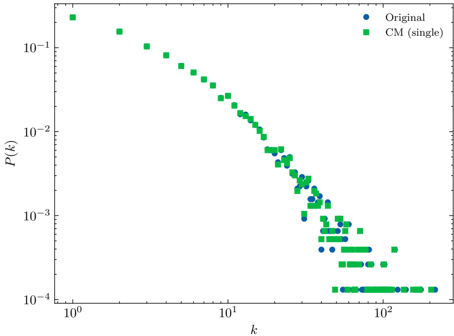
Degree distribution P(k)
