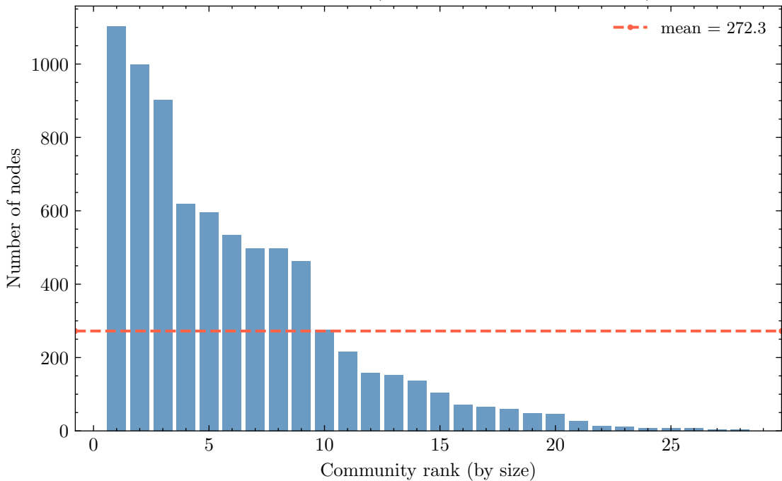
Community sizes ( Q = 0.815 , 28 communities)
