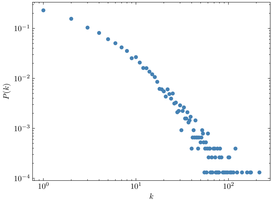
Degree distribution (log-log)
