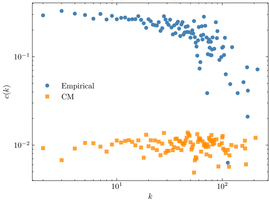
Clustering spectrum: empirical vs CM
