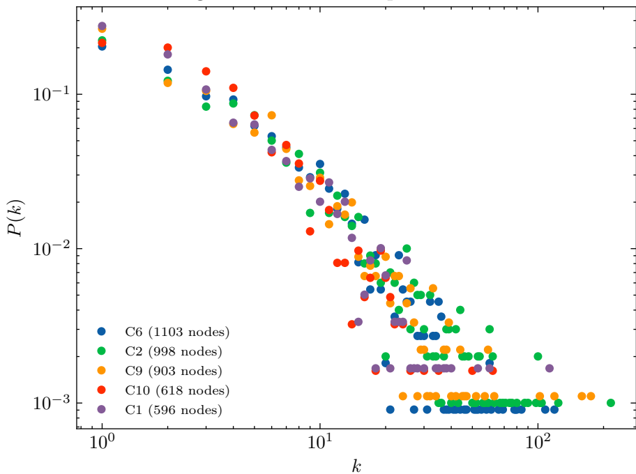
Degree distribution: top 5 communities
