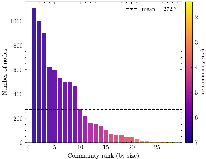
Community sizes ( Q = 0.815 , 28 communities)
