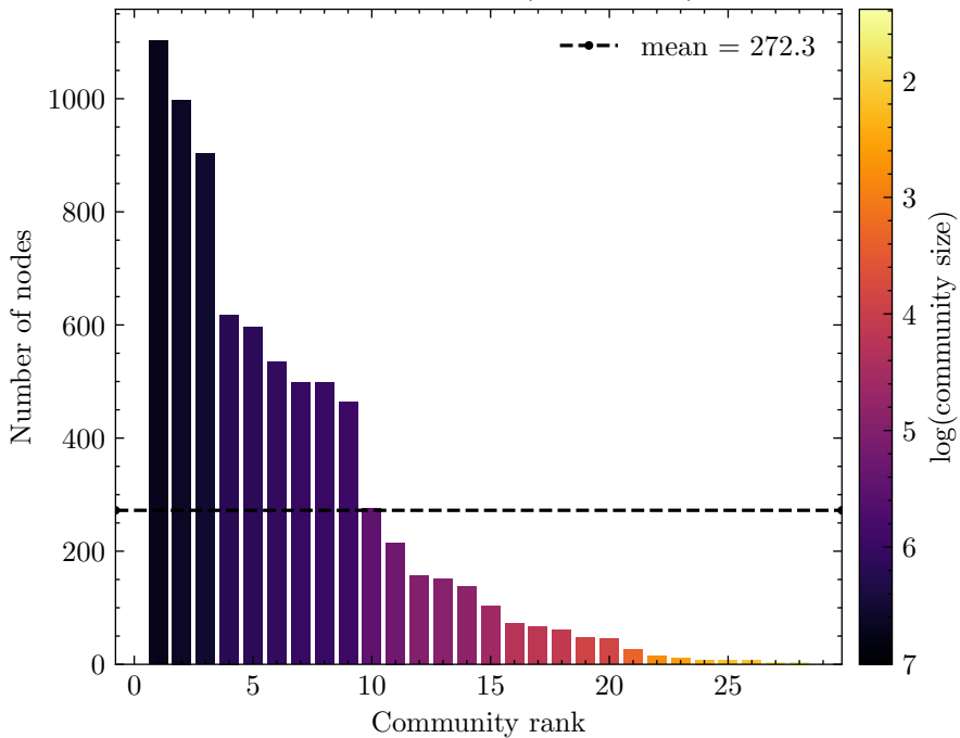
Community sizes ( Q = 0.815 )
