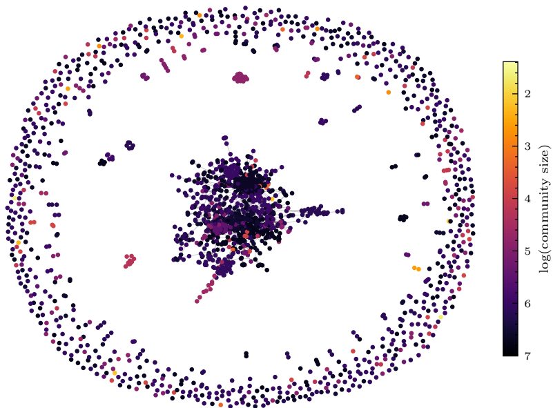
Louvain communities (sampled 1999 / 7624 nodes) Q = 0.8148 , 28 communities
