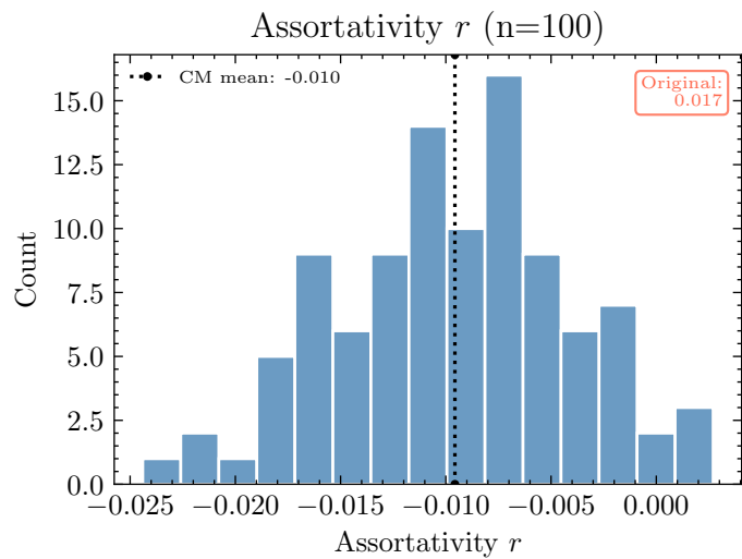
CM ensemble distributions (100 realizations)
