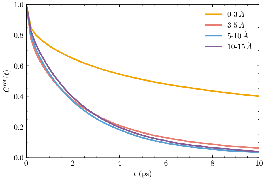
Rotational correlation for T = 290.5 K
