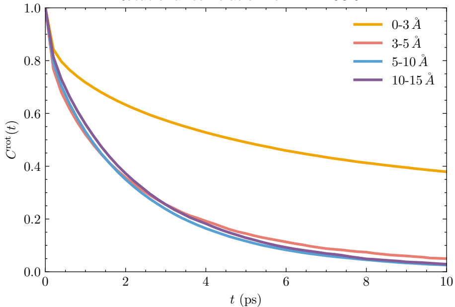
Rotational correlation for T = 293.5 K
