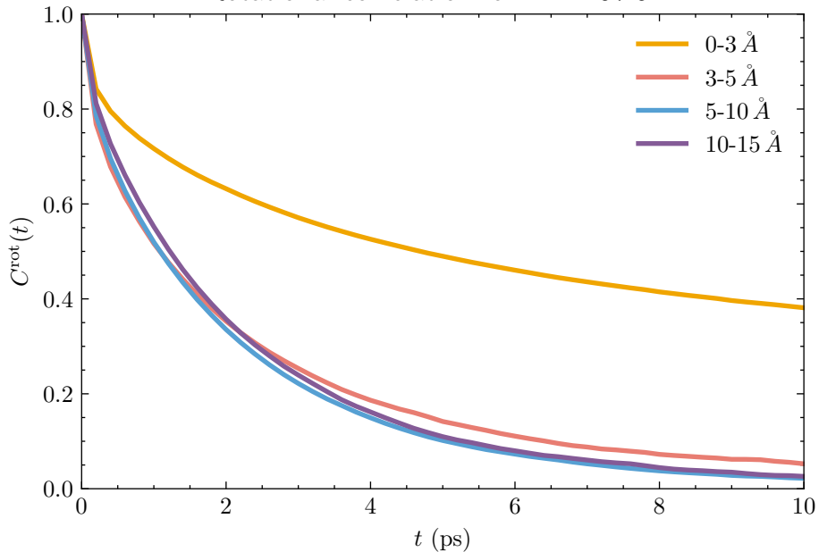
Rotational correlation for T = 297.5 K
