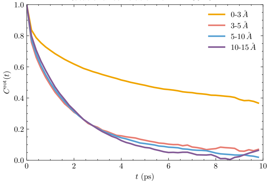
Rotational correlation for T = 304.5 K
