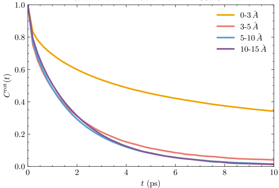
Rotational correlation for T = 307.5 K
