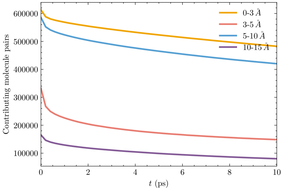
Shell population — T = 290.5 K
