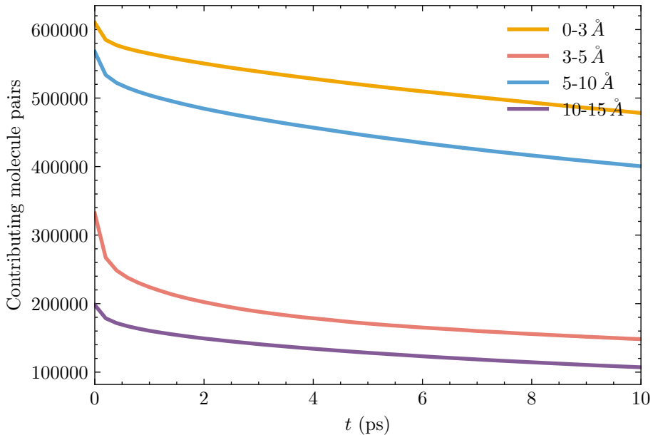
Shell population — T = 293.5 K
