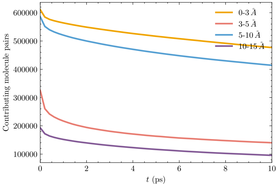
Shell population — T = 297.5 K
