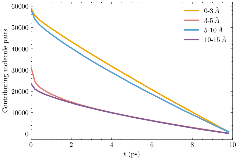
Shell population — T = 304.5 \text{ K}
