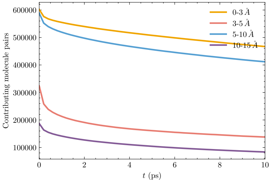
Shell population — T = 307.5 K
