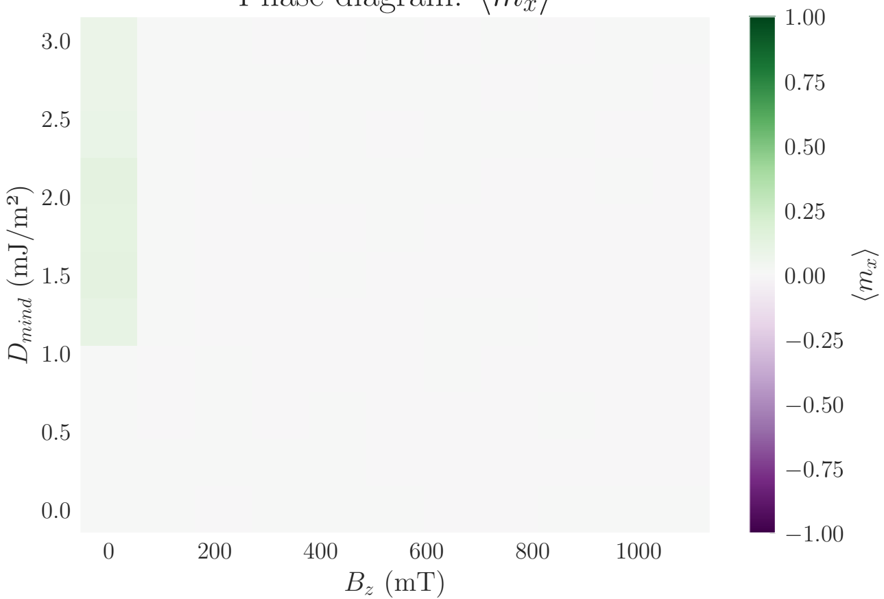
Phase diagram: \langle m_x \rangle
