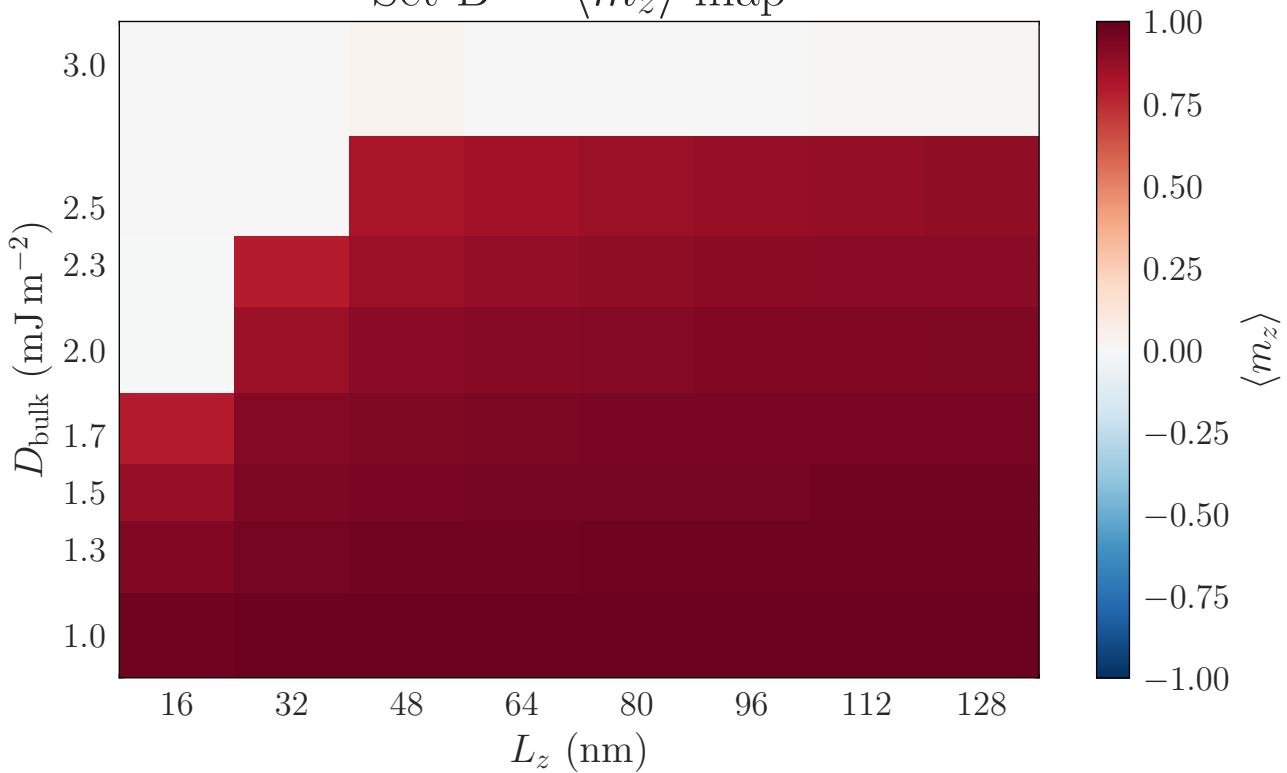
Set B — \langle m_z \rangle map
