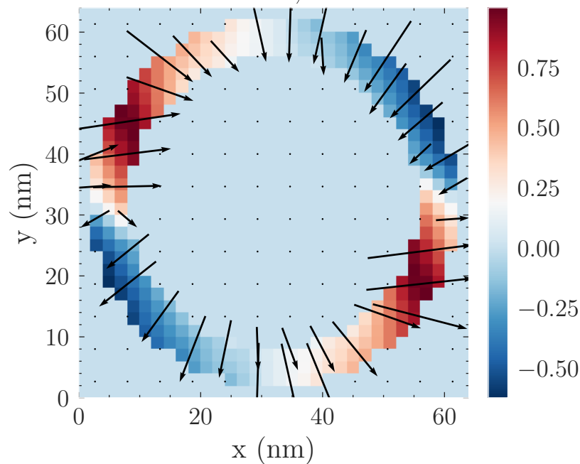
mx + arrows, z=81 nm
