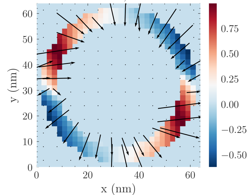
mx + arrows, z=121 nm
