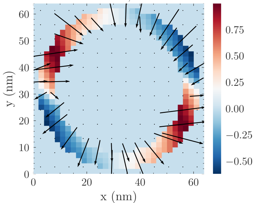
mx + arrows, z=41 nm
