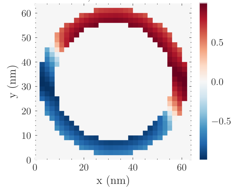
mx + arrows, z=121 nm
