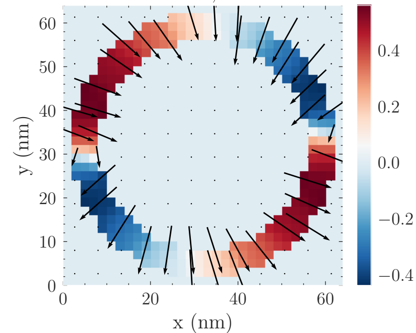
mx + arrows, z=121 \text{ nm}
