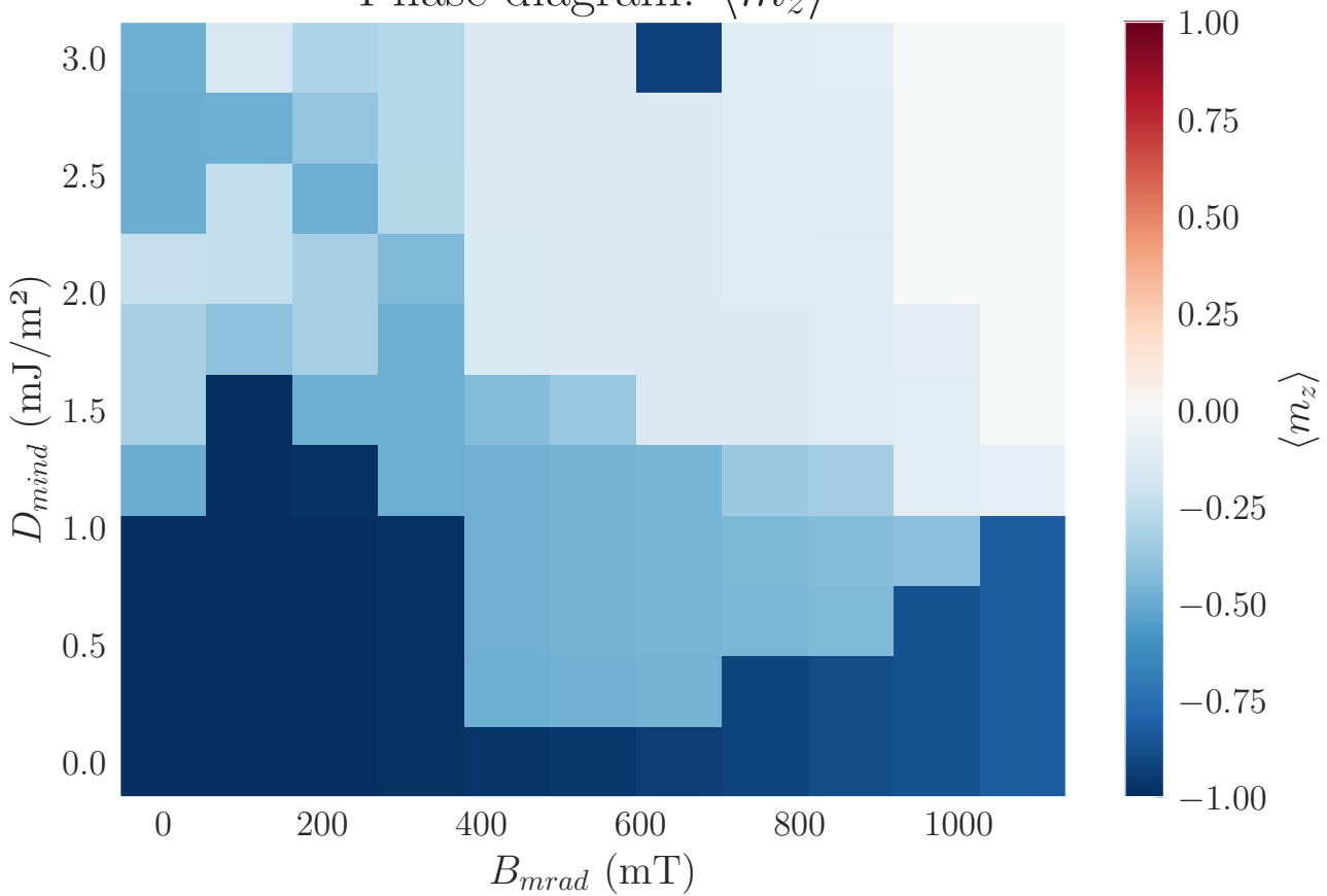
Phase diagram: \langle m_z \rangle
