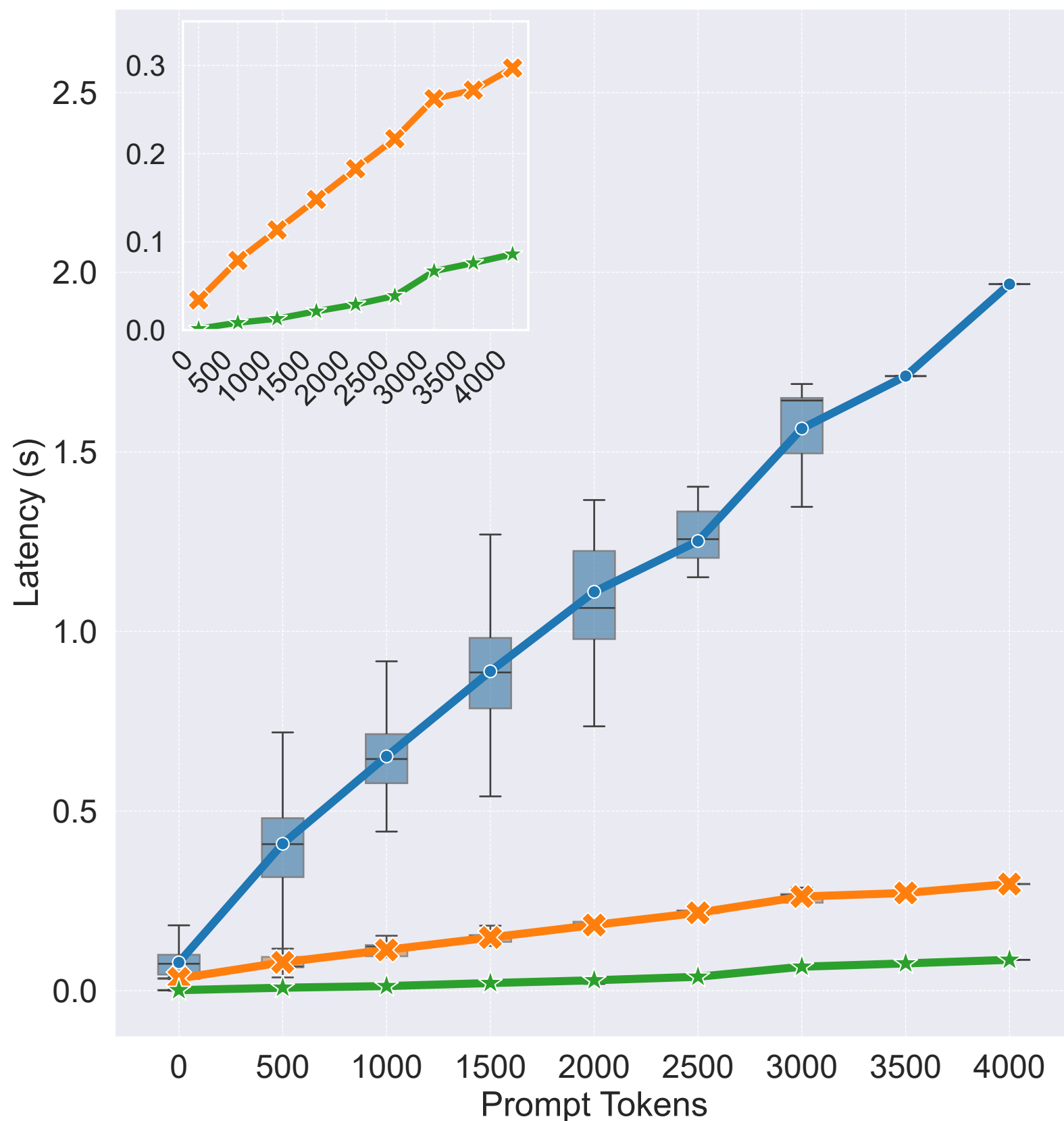
(a) Compression latency across baselines
