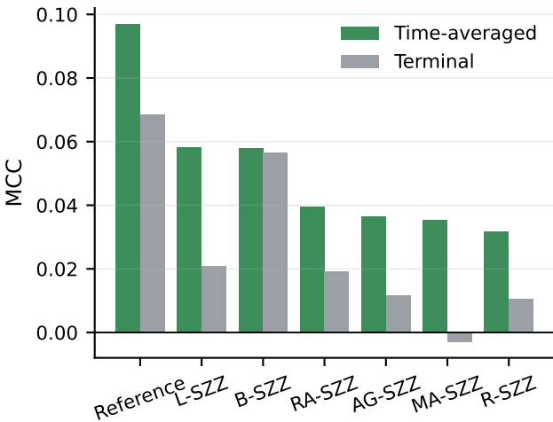
(a) Mean MCC by training labels
