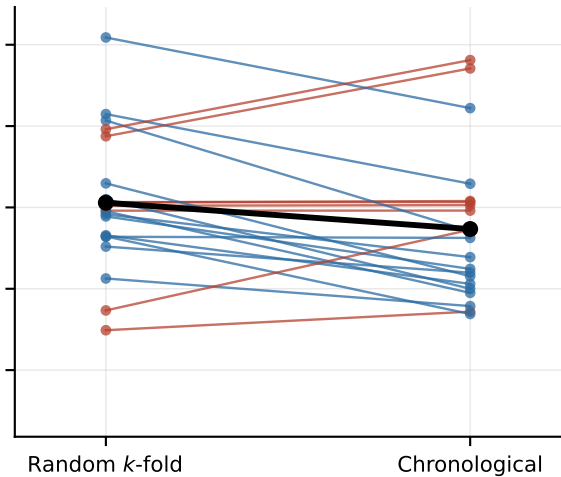
(b) LAPredict
