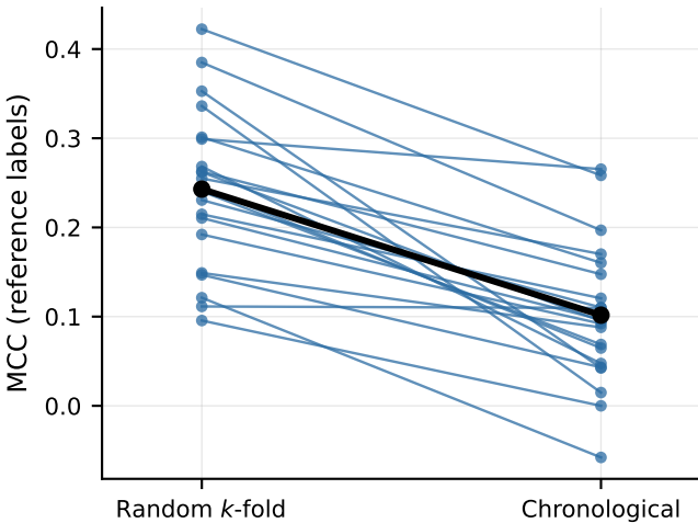
(a) JITLine
