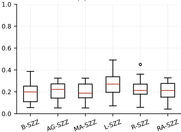
(a) Precision
