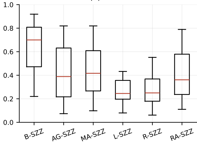
(b) Recall
