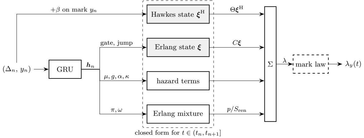
Figure 1: EPT-X at one event. The GRU summary \mathbf{h}_n sets the jump of the neural Erlang state, the hazard parameters and the renewal weights, while the Hawkes state is driven by the event mark alone. The grey boxes are the states carried from one event to the next. Until the next event, all four terms evolve in closed form. The dashed box is the optional residual mark law, which splits the total intensity across marks without changing it.
