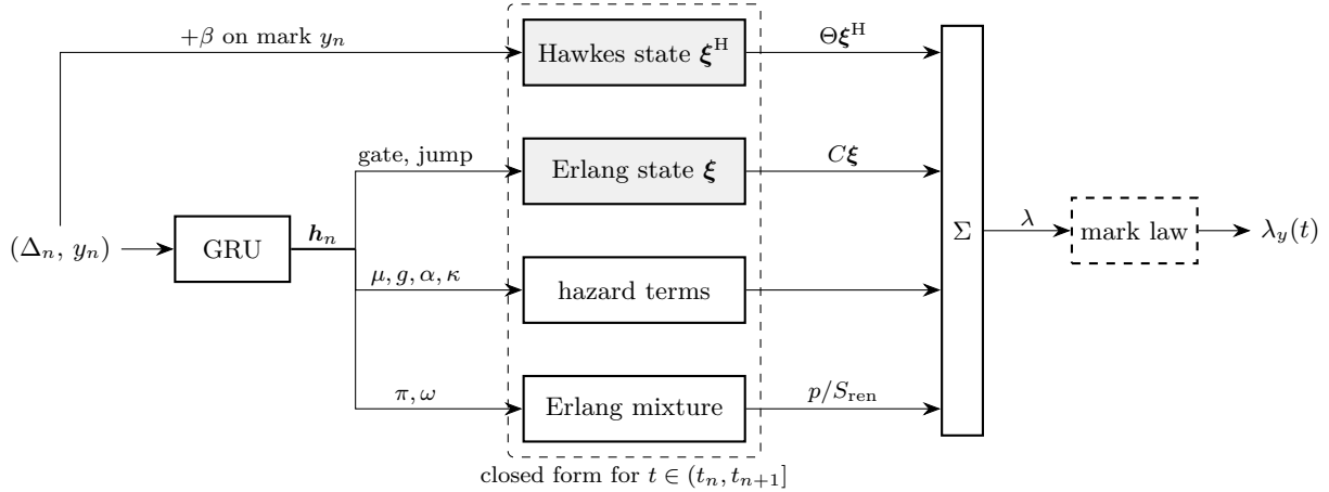
Figure 1: EPT-X at one event. The GRU summary h_n sets the jump of the neural Erlang state, the hazard parameters and the renewal weights, while the Hawkes state is driven by the event mark alone. The grey boxes are the states carried from one event to the next. Until the next event, all four terms evolve in closed form. The dashed box is the optional residual mark law, which splits the total intensity across marks without changing it.
