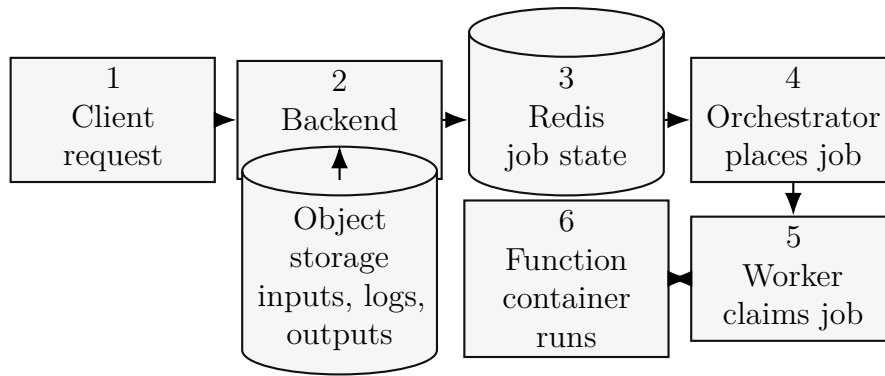
Figure 6.1: Asynchronous invocation execution path. The backend owns artifact storage. The orchestrator owns Redis coordination. The worker runs the function and reports completion.
