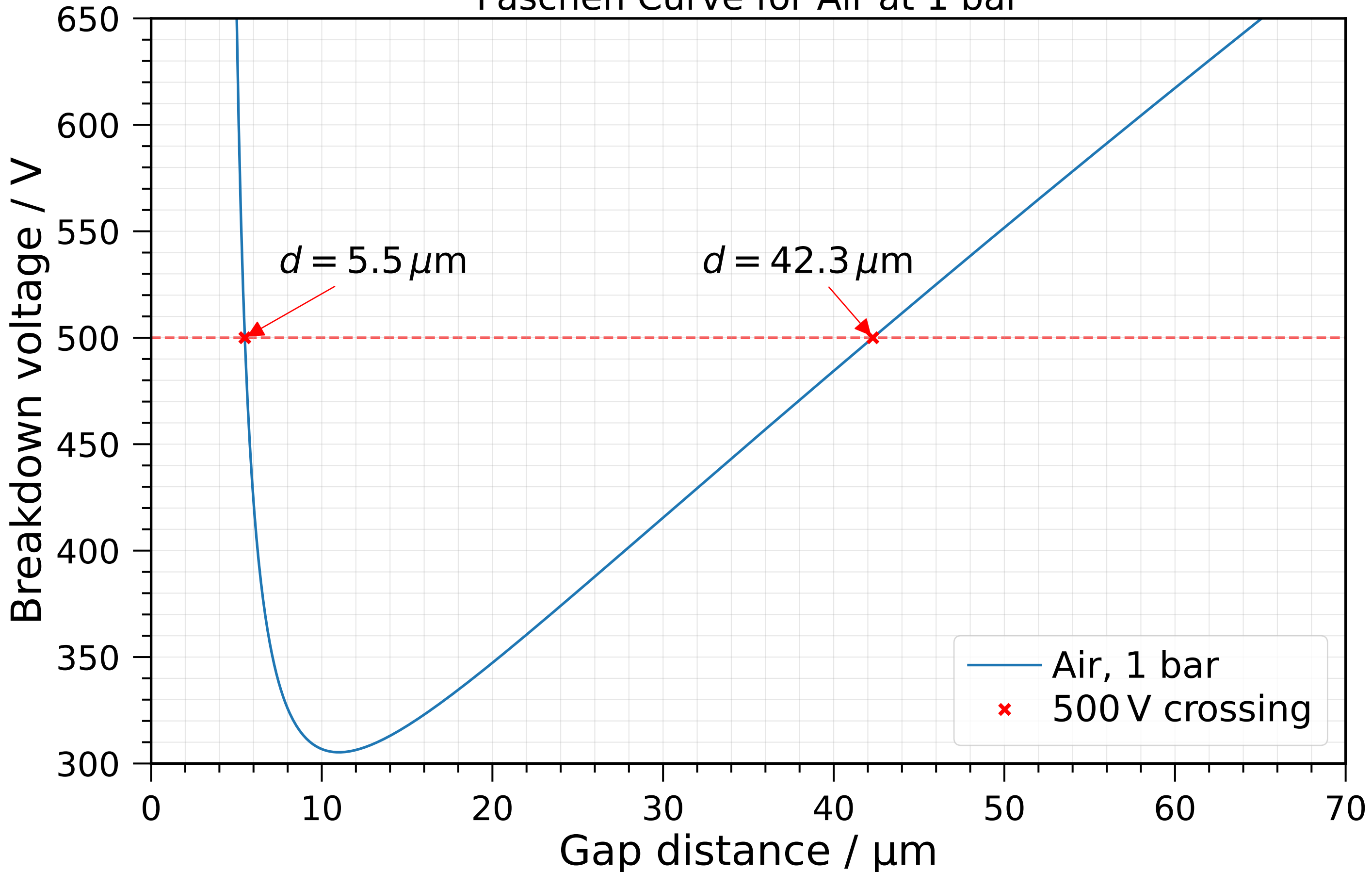
Paschen Curve for Air at 1 bar
