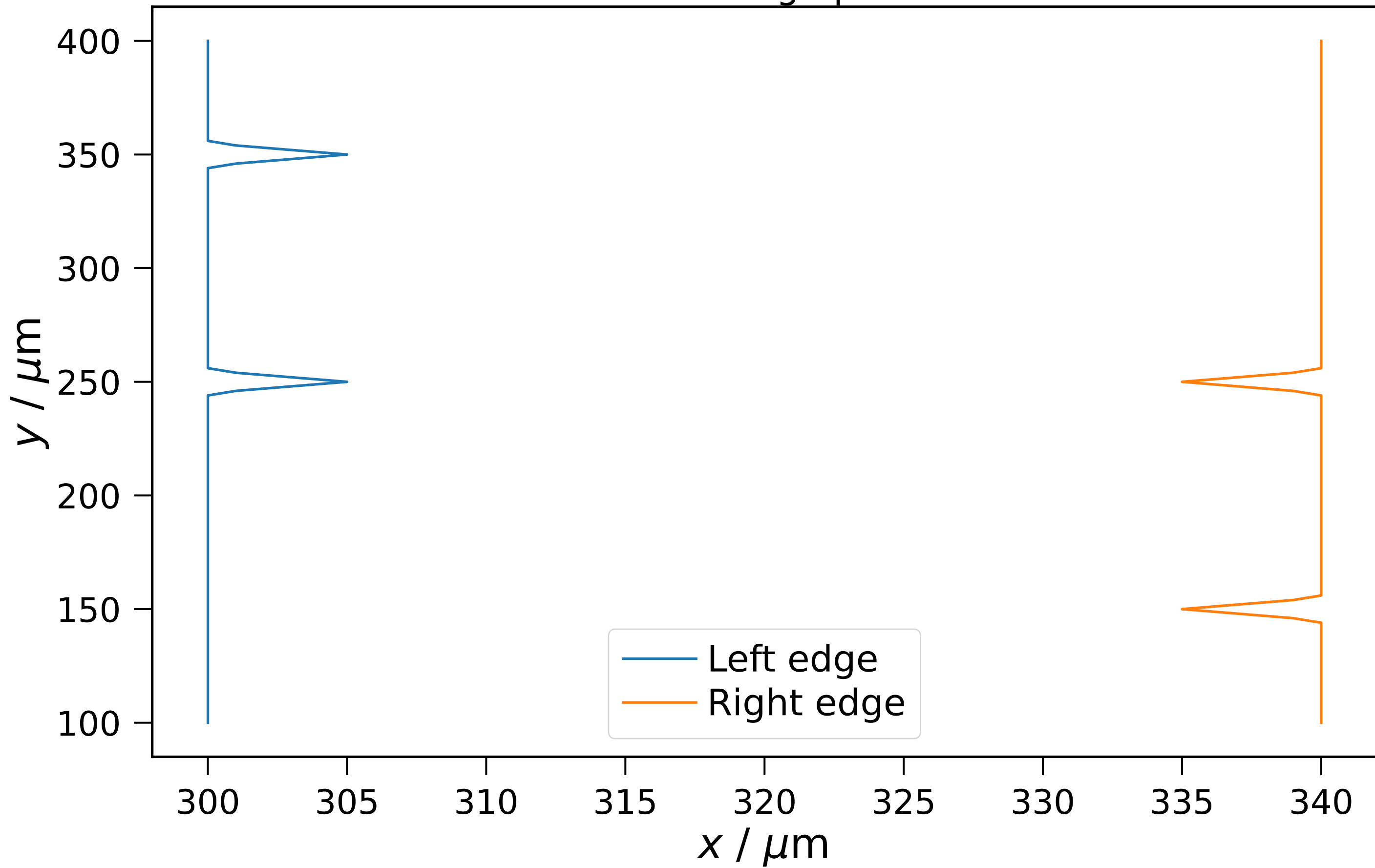
Serrated edge profiles
