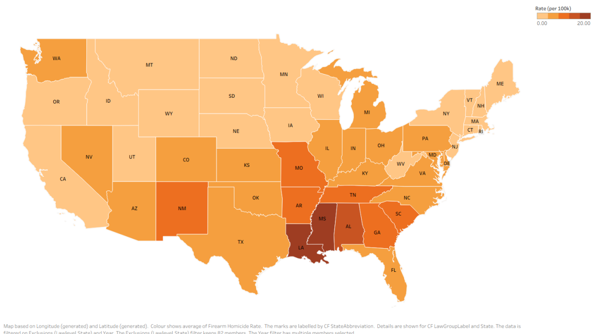
Firearm Homicide Rate by State (2023)
