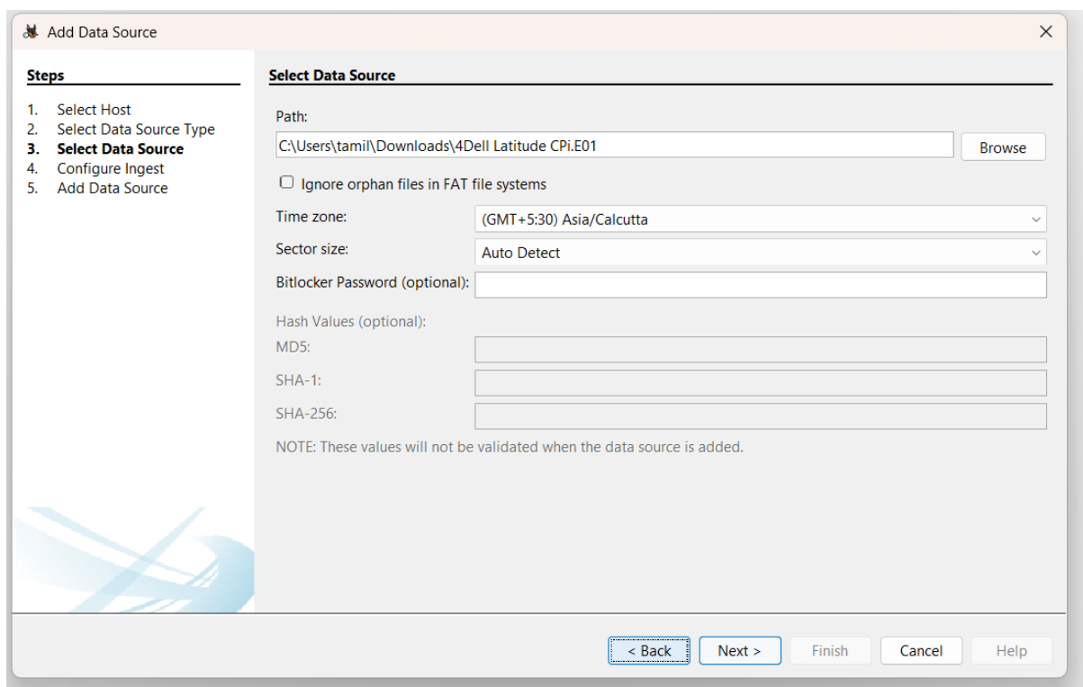
Figure 4: Importing the .E01 evidence file data source
