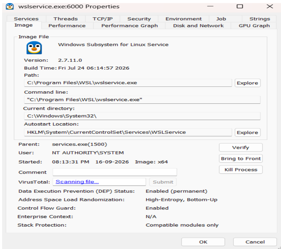
Figure 3: Inspecting image properties, cryptographic signatures, and execution file paths
