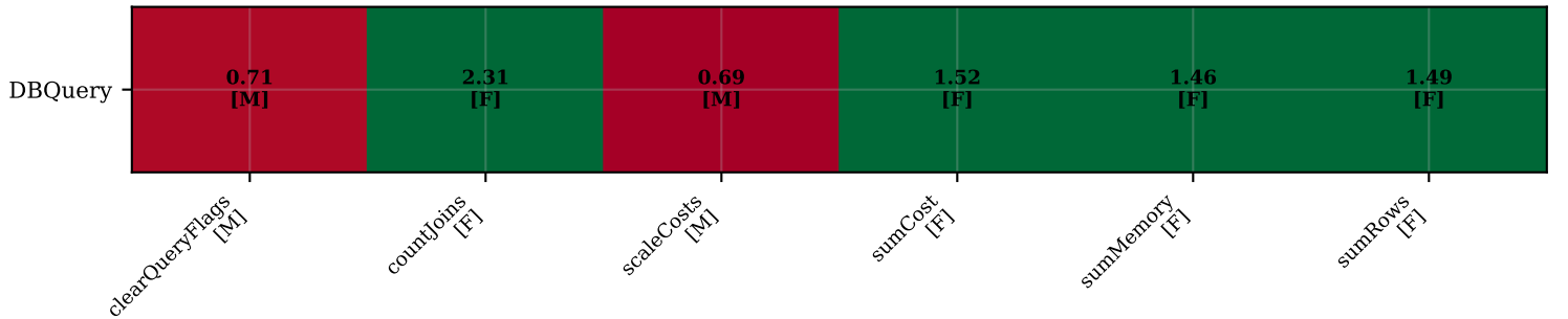
DBQuery: per-pass speedup heatmap (F=fold M=map ?=unknown | SoA=13 buffers total)
