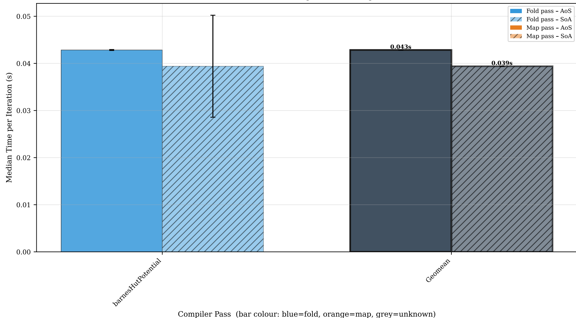
OctTree_barnesHutPotential — AoS (solid) vs SoA (hatched), all passes (error bars = std dev, rightmost bar = geomean)
