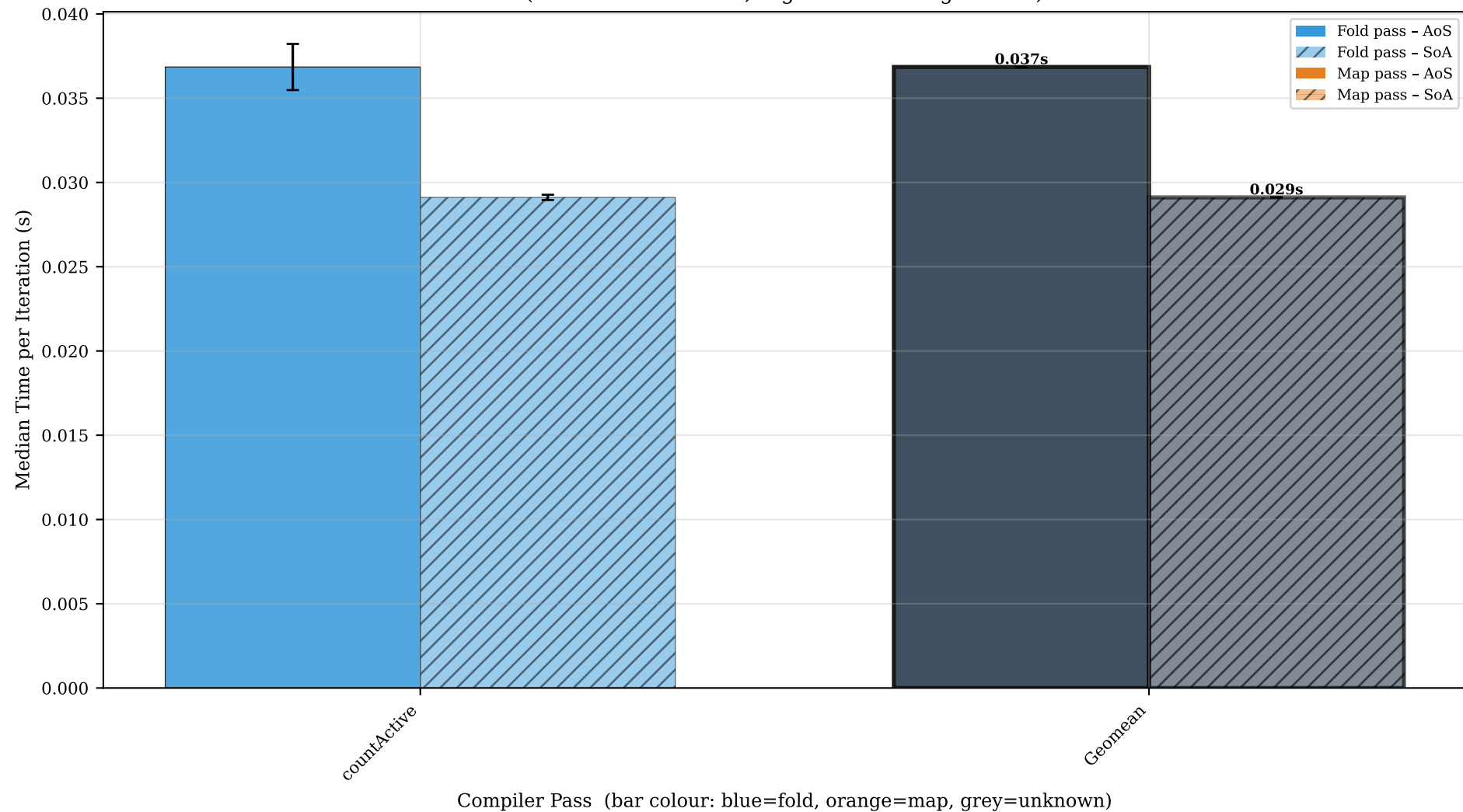
OctTree_countActive — AoS (solid) vs SoA (hatched), all passes (error bars = std dev, rightmost bar = geomean)
